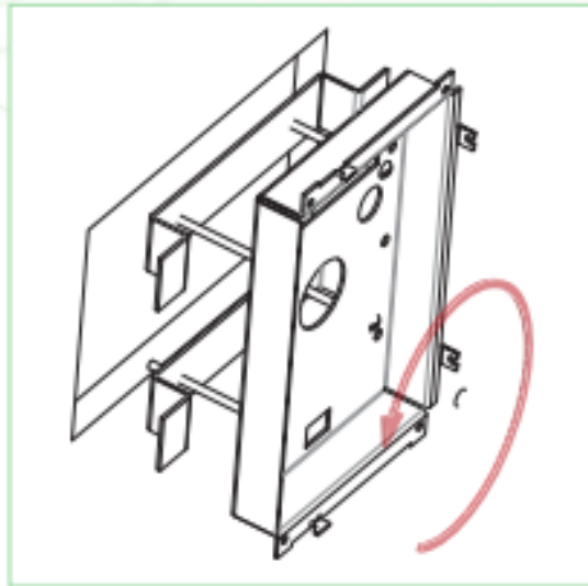
Inserting and Rotating in Wall
