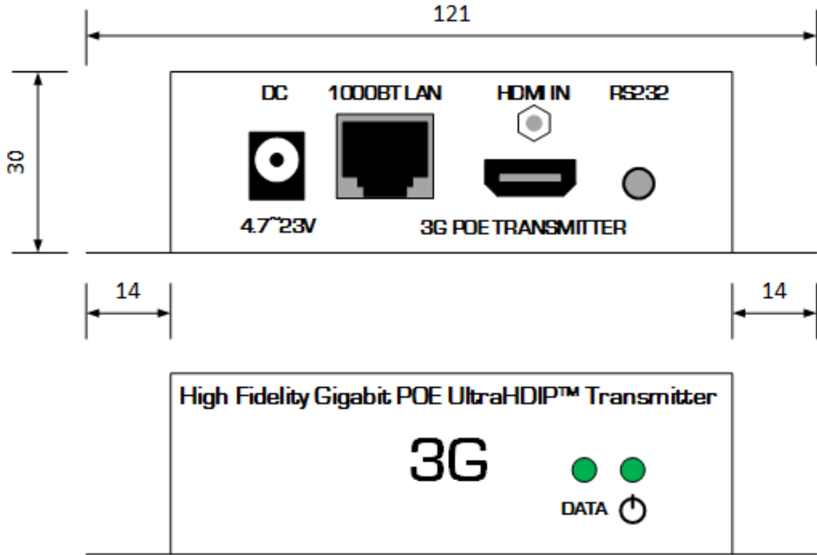
707PoE Front/Back
