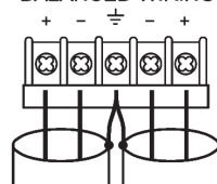
BALANCED WIRING
