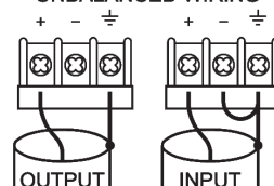
UNBALANCED WIRING
